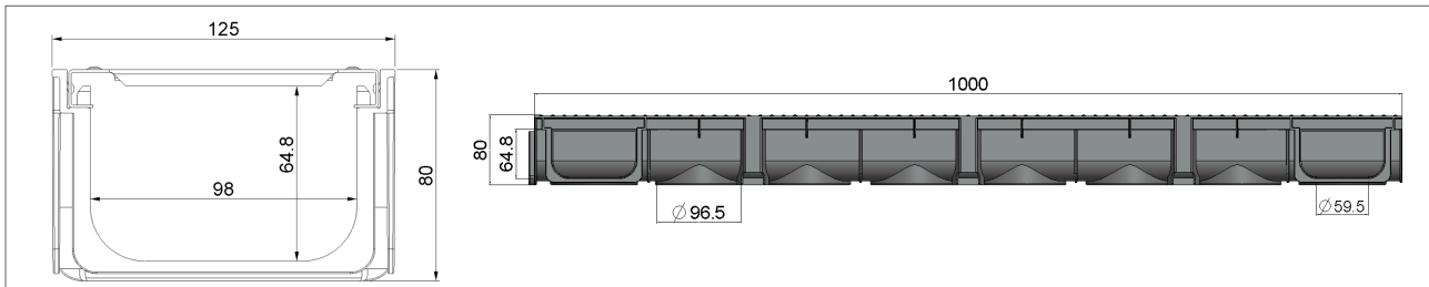
Technical sections of Plastic drain channel with galvanized grating
